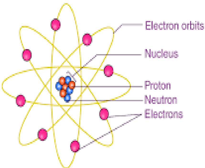
The Structure of Atom
